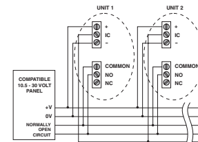
Figure 6a Circuit for Normally Open Relay Contacts
