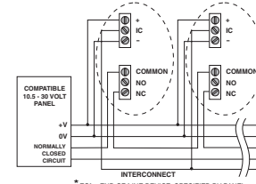
Figure 6b Circuit for Normally Closed Relay Contacts
