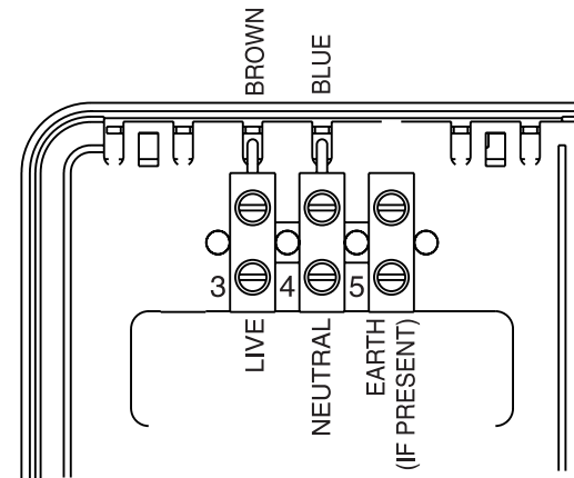
Figure 6 - Recessed Wiring
